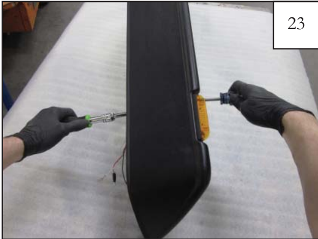
Secure the side marker light to the outer flare with Screw (SW1-0054), Nut (NU1-0018) and Washer (WA1-0003) using a #2 Phillips bit and a 11/32" socket with 6" extension. (2 places) NOTE: If you are having trouble putting the washer and nut on the screw, use needle nose pliers.
