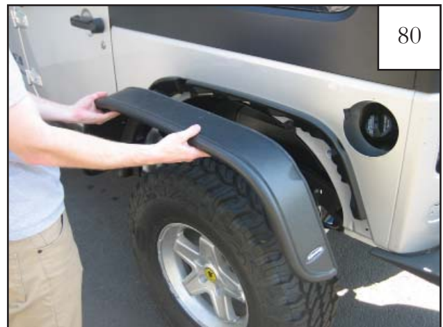
Place the outer flare over the inner pieces and push until snug against the vehicle surface. Make sure splash shield is tucked behind flare.
